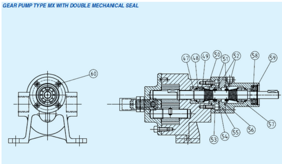
GEAR PUMP TYPE MX WITH DOUBLE MECHANICAL SEAL
