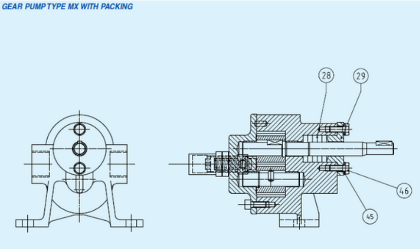
GEAR PUMP TYPE MX WITH PACKING
